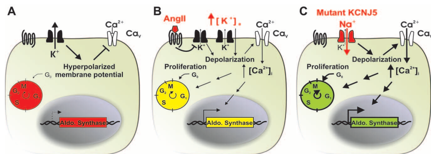
Fig. 4. Proposed mechanism underlying aldosterone-producing adenoma and Mendelian aldosteronism. (A) Adrenal glomerulosa cells have a high resting K^+ conductance, which produces a highly negative membrane potential (2). (B) Membrane depolarization by either elevation of extracellular K^+ or closure of K^+ channels by angiotensin II activates voltage-gated Ca^{2+} channels, increasing intracellular Ca^{2+} levels (1). This provides signals for increased expression of enzymes required for aldosterone biosynthesis, such as aldosterone synthase, and for increased cell proliferation. (C) Channels containing KCNJ5 with G151R, T158A, or L168R mutations conduct Na^+ , resulting in Na^+ entry, chronic depolarization, constitutive aldosterone production, and cell proliferation.
